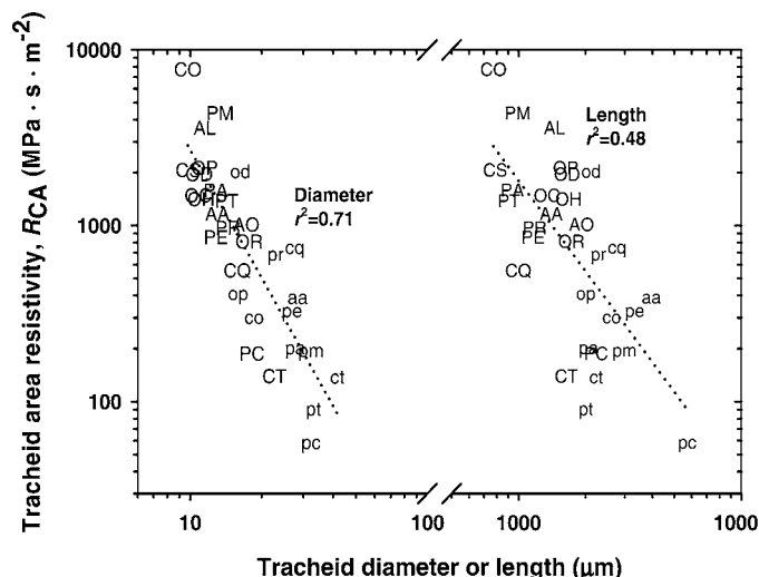
Fig. 1. Tracheid area resistivity ( R_{CA} ) plotted as a function of tracheid diameter, D , or tracheid length, L (SE averaged 24% of R_{CA} , 7% of D , and 3% of L ). Across all species measured, the roots (lowercase letters) typically had wider and longer tracheids than stems (uppercase letters) correspond to species in Table 1; see also Appendix S1 accompanying the online version of this article).
