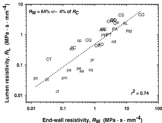
Fig. 2. Lumen resistivity ( R_L ) plotted as a function of end wall resistivity ( R_W ) for all species measured (see Table 1 for species abbreviations; lowercase letters correspond to roots; uppercase letters correspond to stems). Values are expressed on a mean tracheid area basis, with R_W contributing approximately 64% to the total tracheid resistivity ( R_C ). The SE averaged 14% of R_L and 40% of R_W (see also Supplemental Appendix 1 with the online version of this article).
